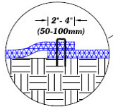
DETAIL 5B "OVERLAP"
