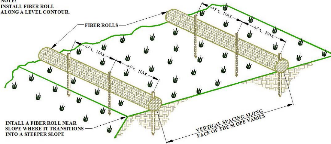
TYPICAL FIBER ROLL INSTALLATION N.T.S.
