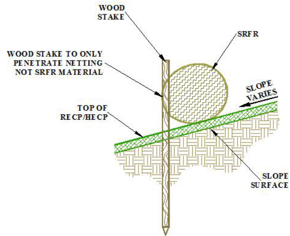
STAKE DETAIL ON TOP OF ECB N.T.S.
