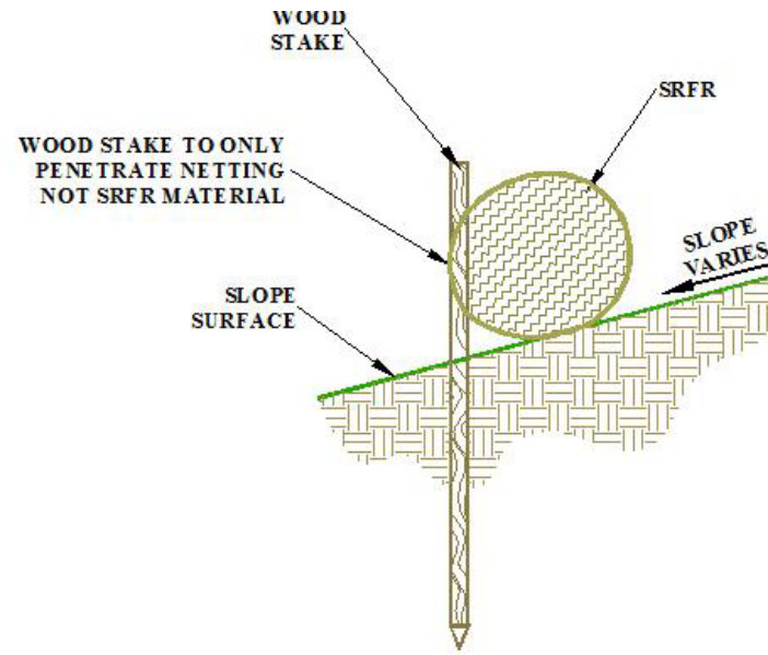
STAKE DETAIL ON BARE SOIL N.T.S.
