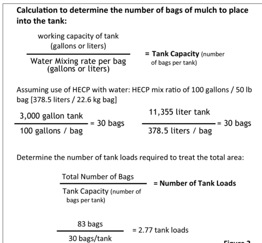
Figure 4. Calculation to Determine Number of Mulch Bags to Put into the Tank.
